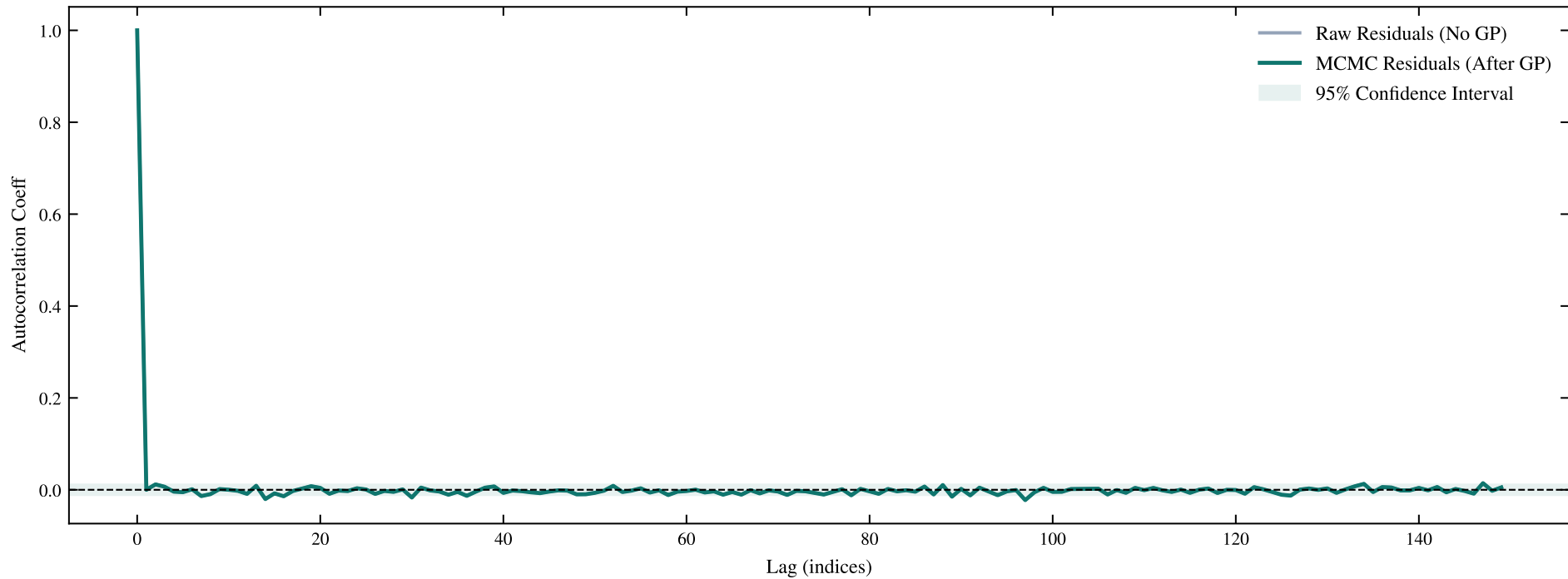
TIC 261369656 | Sectors: 104, 105 | GP Residuals Autocorrelation Function (ACF)
