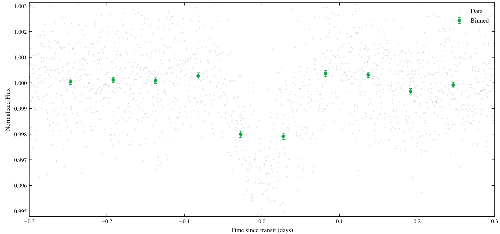
TIC 261369656 | Sectors: 104, 105 | Phase-Folded Transit (P = 10.95861 d)
