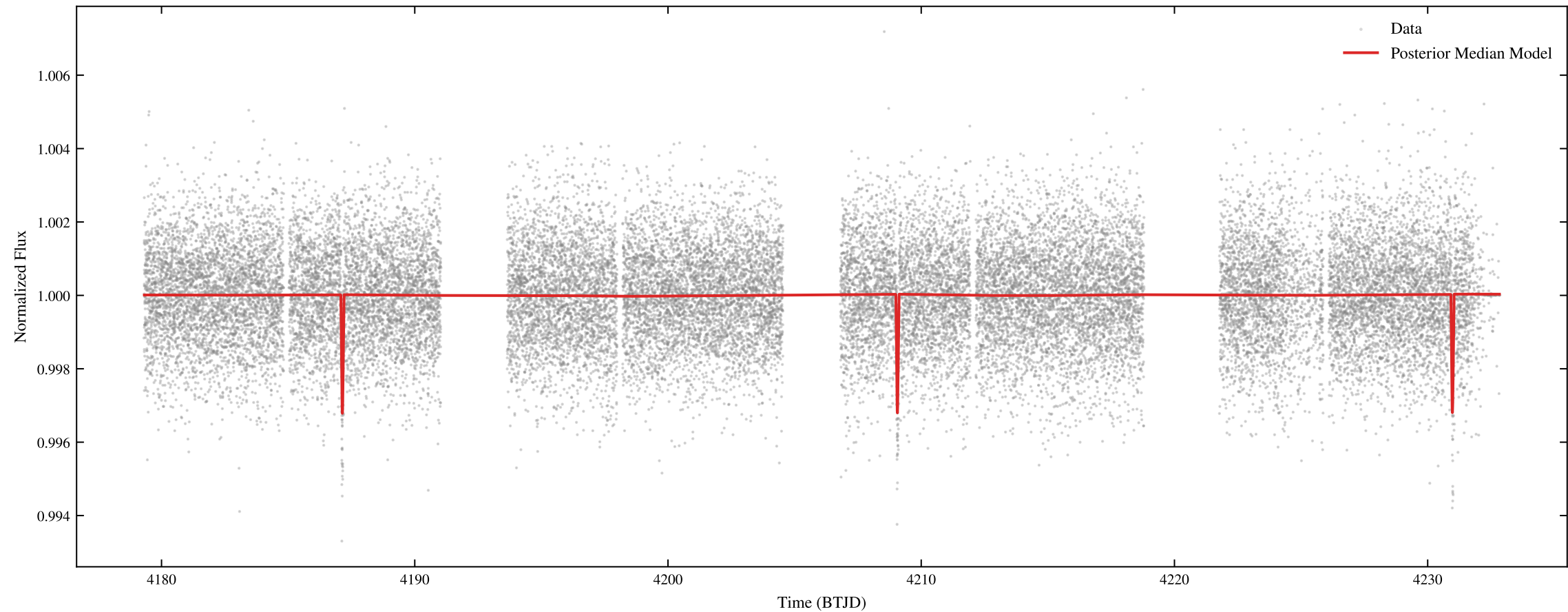
TIC 261369656 | Sectors: 104, 105 | MCMC Posterior Predictive Check
