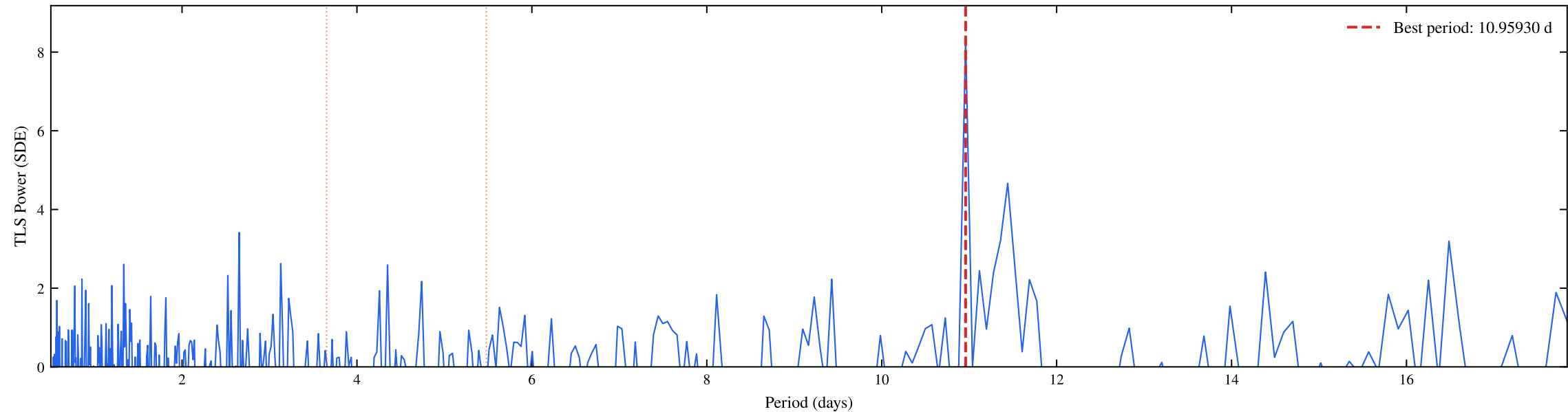
TIC 261369656 | Sectors: 104, 105 | TLS Coarse Periodogram (SDE = 8.34)
