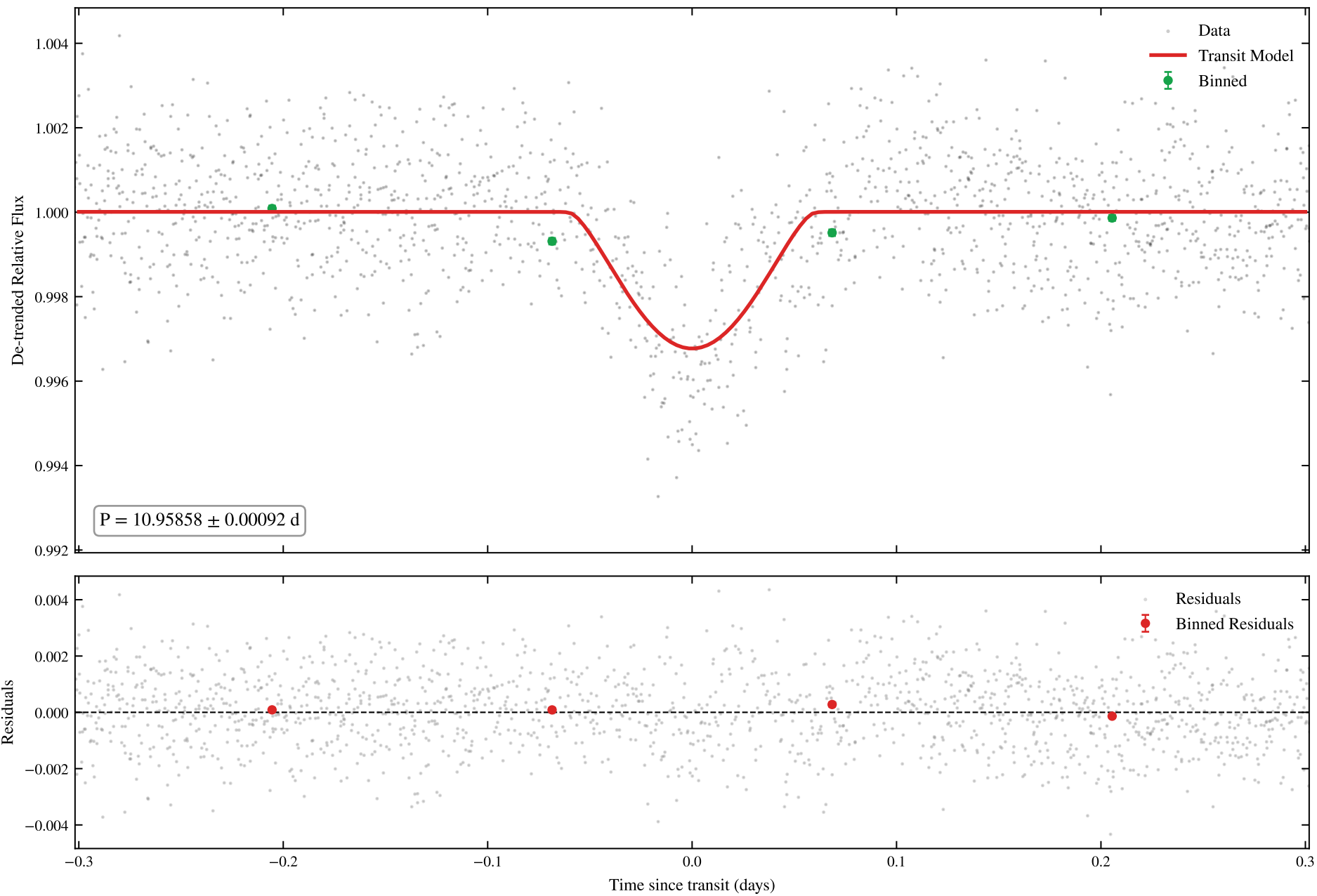
TIC 261369656 | Sectors: 104, 105 | Phased MCMC Fit - Planet 1
