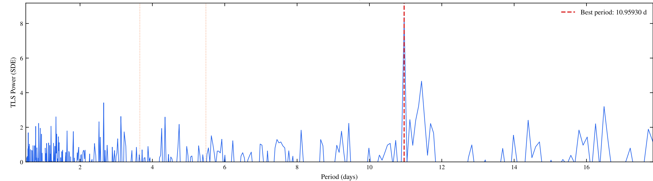
TIC 261369656 | Sectors: 104, 105 | TLS Periodogram (Planet 2 Search) (SDE = 8.34)
