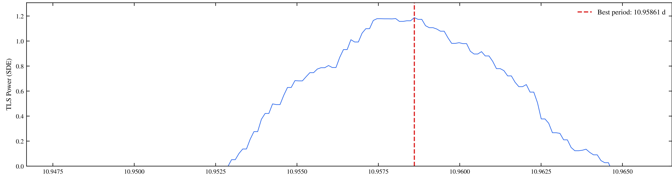
TIC 261369656 | Sectors: 104, 105 | TLS Periodogram (Planet 2 Search) (SDE = 8.34)
