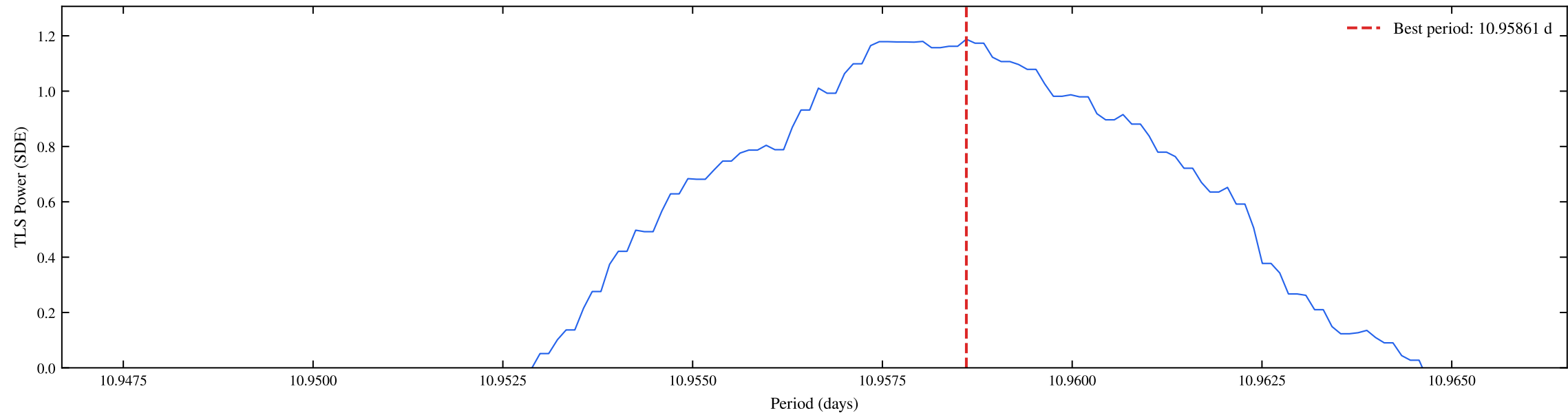
TIC 261369656 | Sectors: 104, 105 | TLS Coarse Periodogram (SDE = 1.19)
