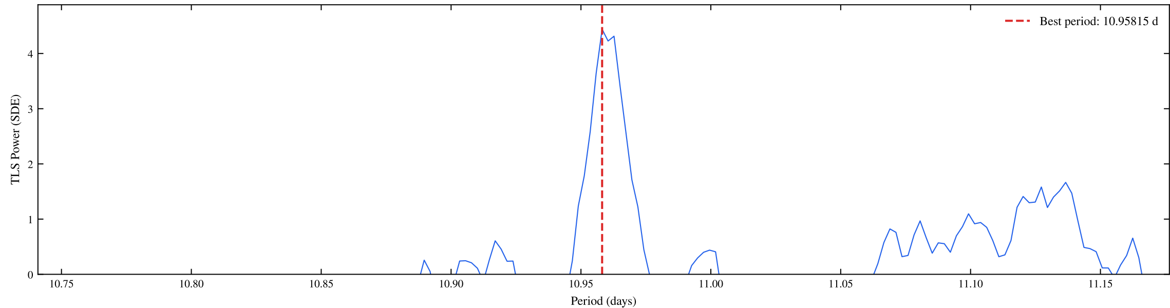
TIC 261369656 | Sectors: 104, 105 | TLS Fine Periodogram (SDE = 4.44)
