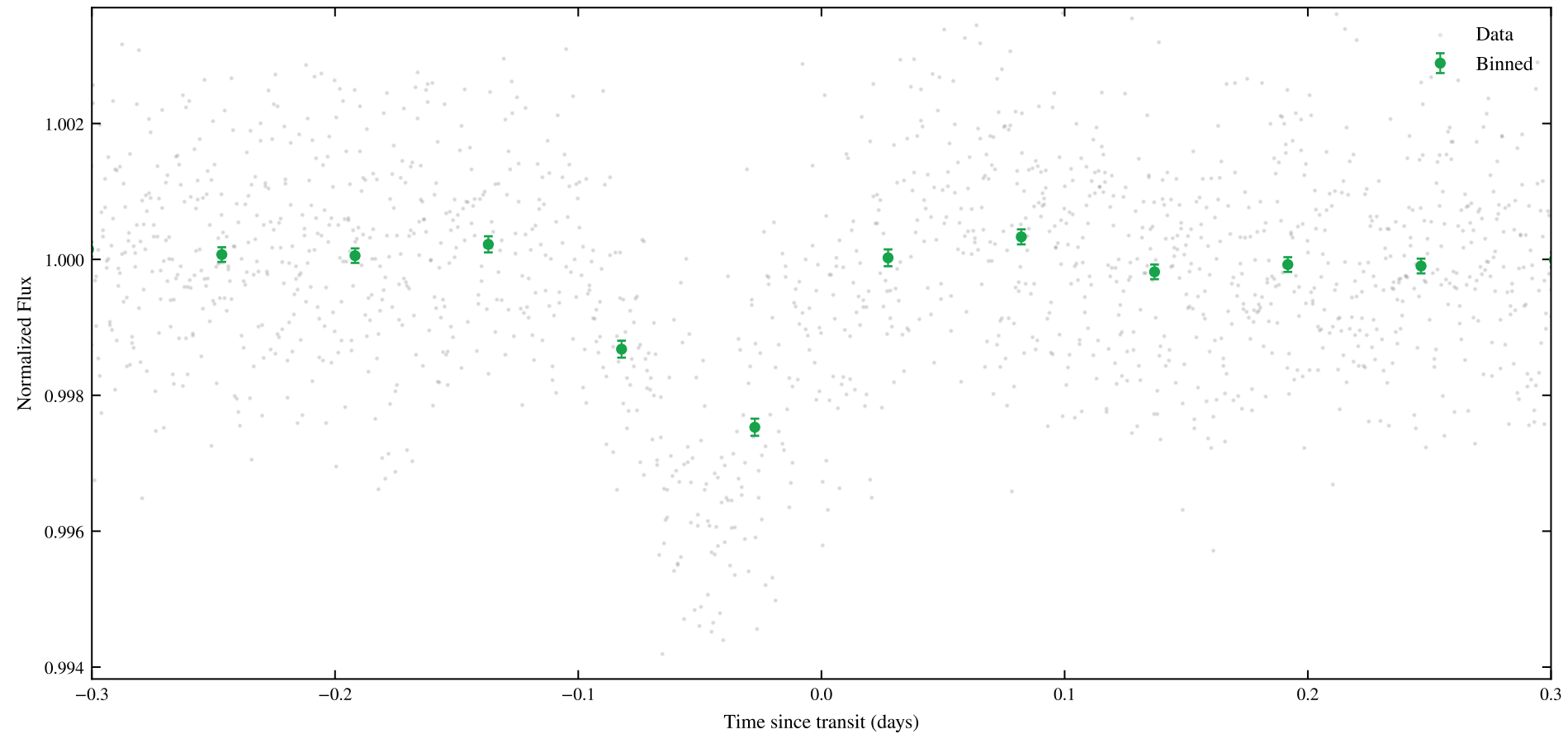
TIC 261369656 | Sectors: 104, 105 | Phase-Folded Transit (P = 10.95815 d)
